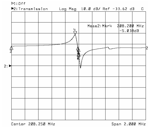
Horizontal: 0.2MHz/Div Vertical: 10dB/Div
