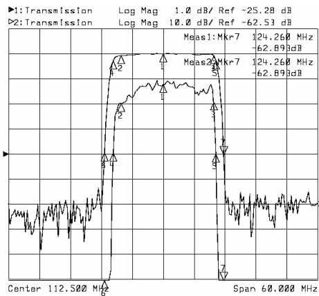
Horizontal: 6.0MHz/Div Vertical: 10dB/Div
