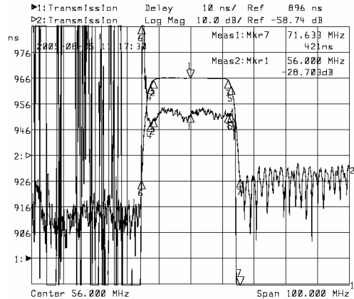
Horizontal: 10MHz/Div Vertical: 10ns/Div
