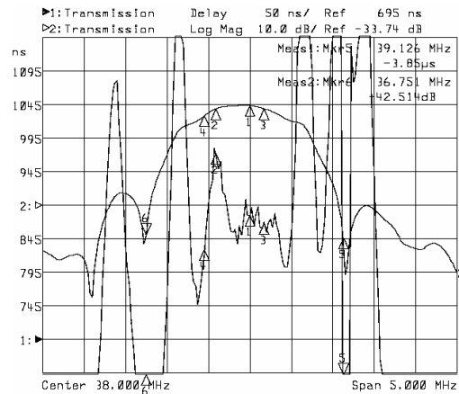
Horizontal: 0.5MHz/Div Vertical: 50nsec/Div
