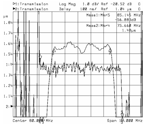
Horizontal: 1.5MHz/Div Vertical: 100nsec/Div
