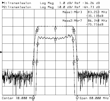
Horizontal: 8MHz/Div Vertical: 10dB/Div
