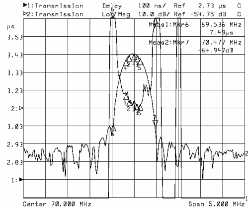
Horizontal: 0.5MHz/Div Vertical: 100ns/Div
