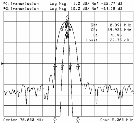
Horizontal: 0.5MHz/Div Vertical: 10dB/Div
