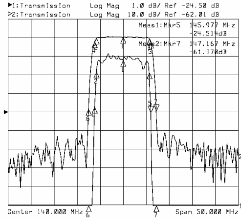
Horizontal: 5.0MHz/Div Vertical: 10dB/Div
