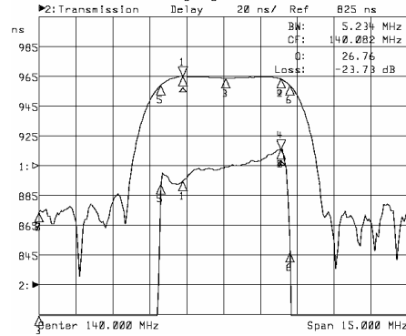
Horizontal: 1.5MHz/Div Vertical: 20nsec/Div
