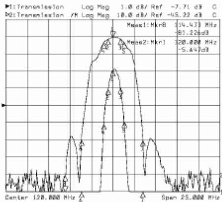
Horizontal: 2.5MHz/Div Vertical: 10dB/Div
