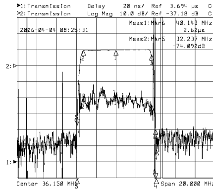
Horizontal: 2MHz/Div Vertical: 10dB/Div&20nsec/Div
