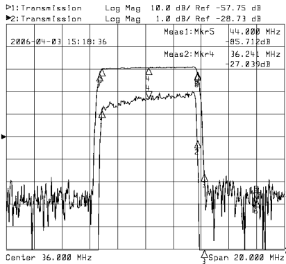
Horizontal: 2MHz/Div Vertical: 10dB/Div&1dB/Div
